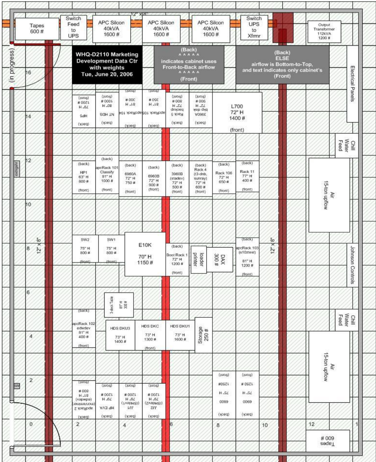
WHQ Building D Computer Room Floor Plan
